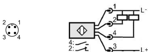
PNP NO i NC
