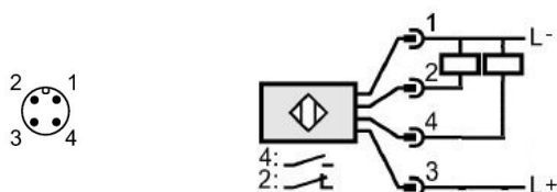
PNP NO i NC
