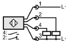
NPN NO i NC
