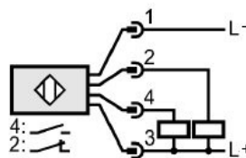
NPN NO i NC
