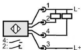
PNP NO i NC
